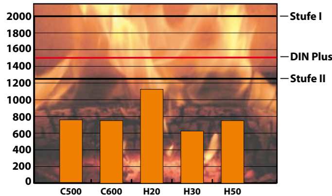
Emissionswerte CO 13% O 2 (mg/Nm 3 )
