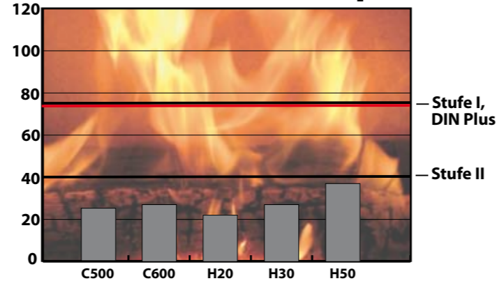
Emissionswerte Feinstaub 13% O 2 (mg/Nm 3 )
